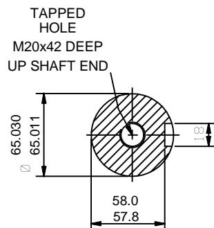
SECTION THROUGH SHAFT EXTENSION (SCALE 1:3)
